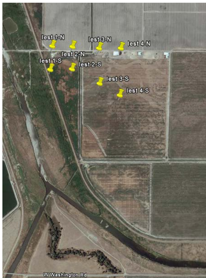
Figure 3: Property 3 Electrical Resistivity Tomography Lines
